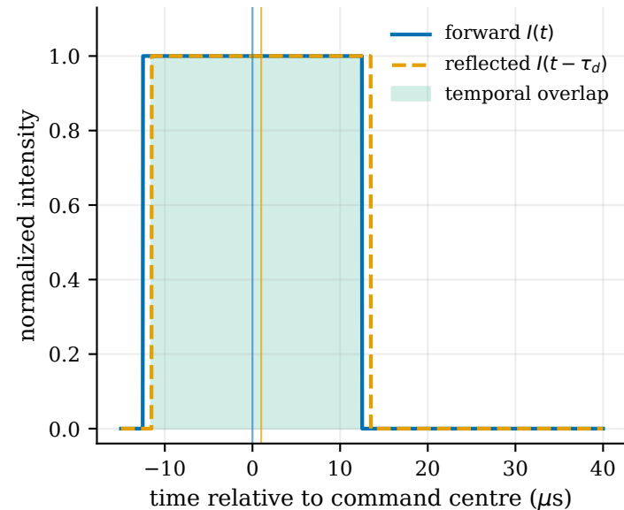
a Counter-propagating envelopes
