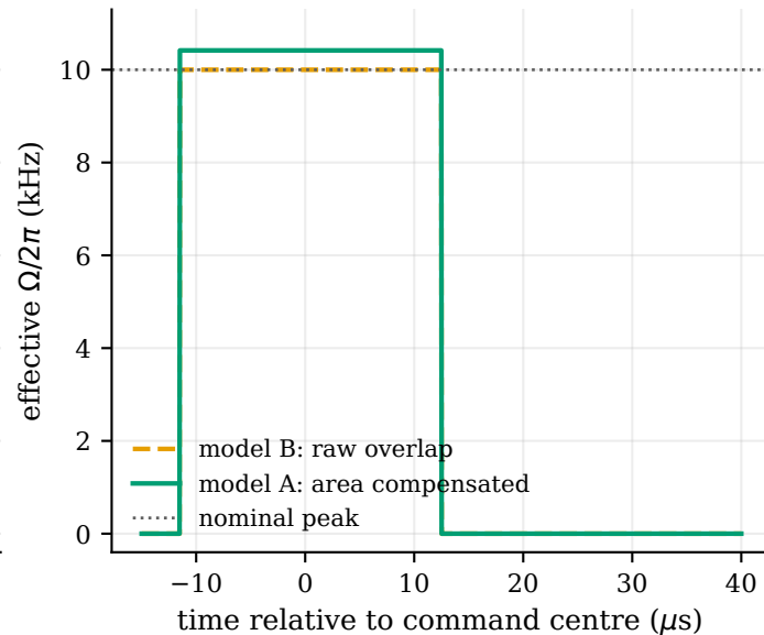
b Effective \pi/2 Rabi pulse
